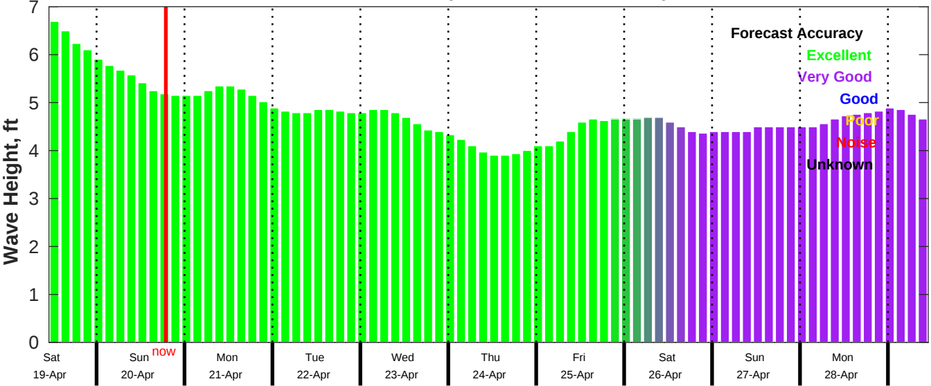
CMEMS Wave Forecast for NDBC 52213 from 18-Apr-2025 11:00:00 to 28-Apr-2025 11:00:00
