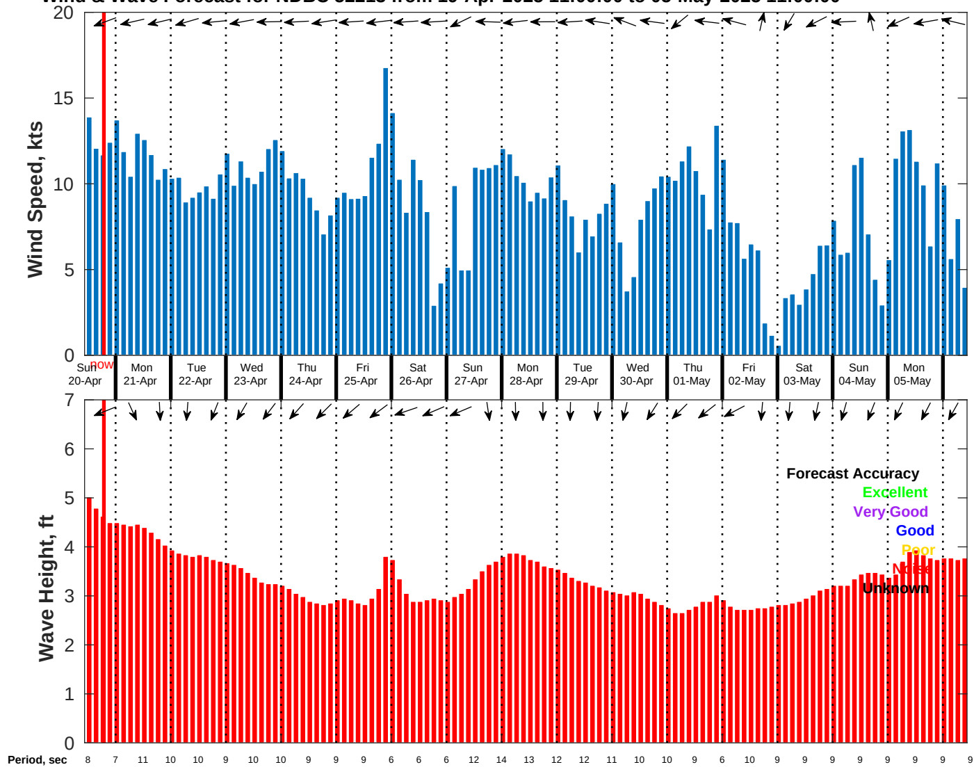
Wind & Wave Forecast for NDBC 52213 from 19-Apr-2025 11:00:00 to 05-May-2025 11:00:00
