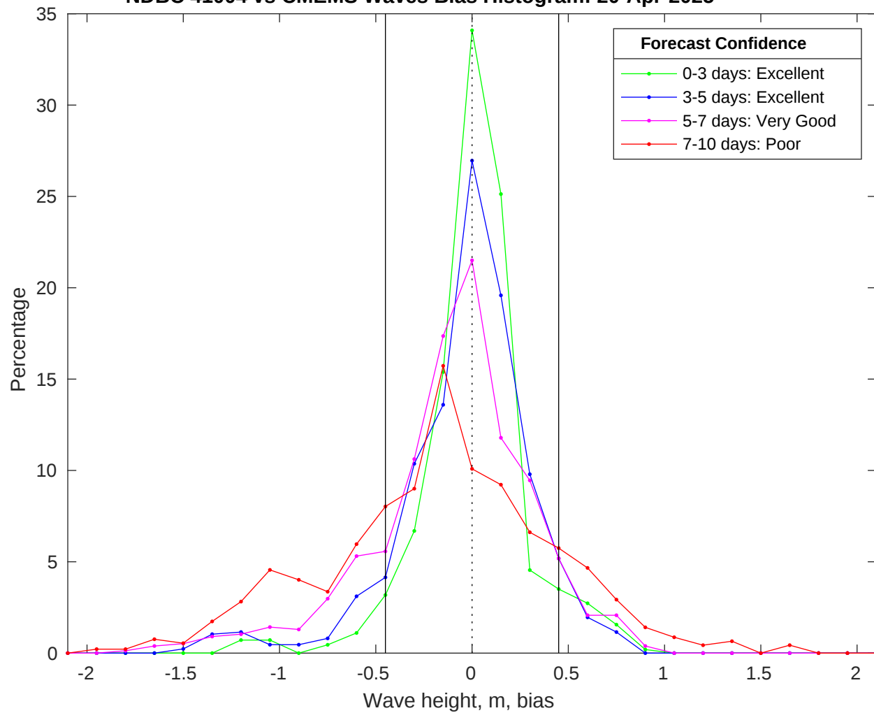
NDBC 41004 vs CMEMS Waves Bias Histogram: 20-Apr-2025
