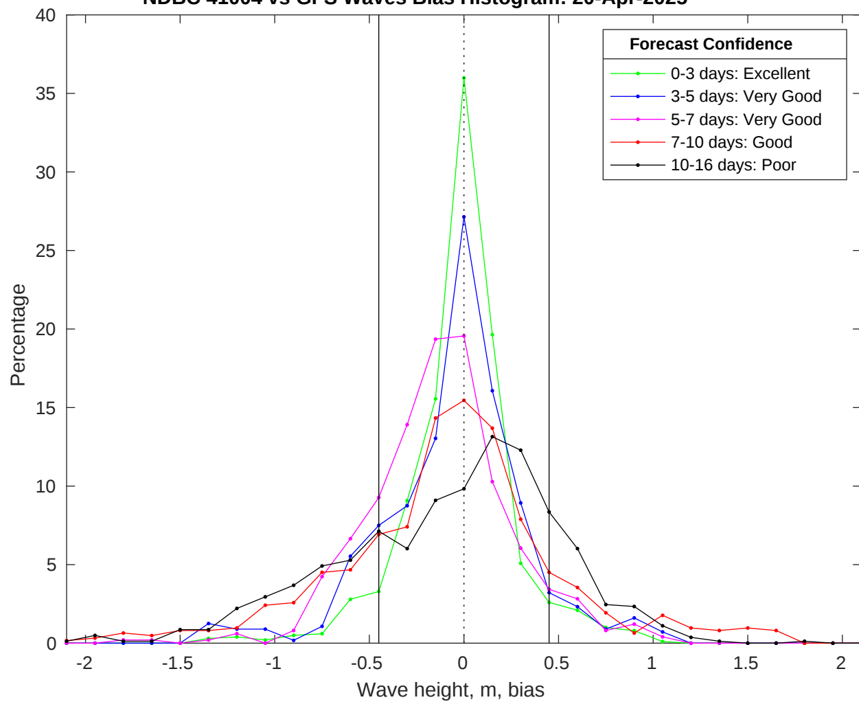
NDBC 41004 vs GFS Waves Bias Histogram: 20-Apr-2025
