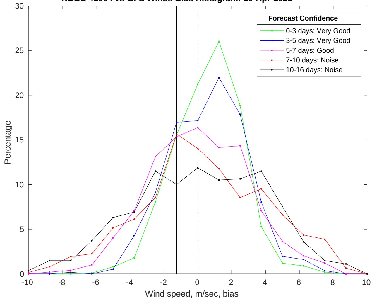
NDBC 41004 vs GFS Winds Bias Histogram: 20-Apr-2025
