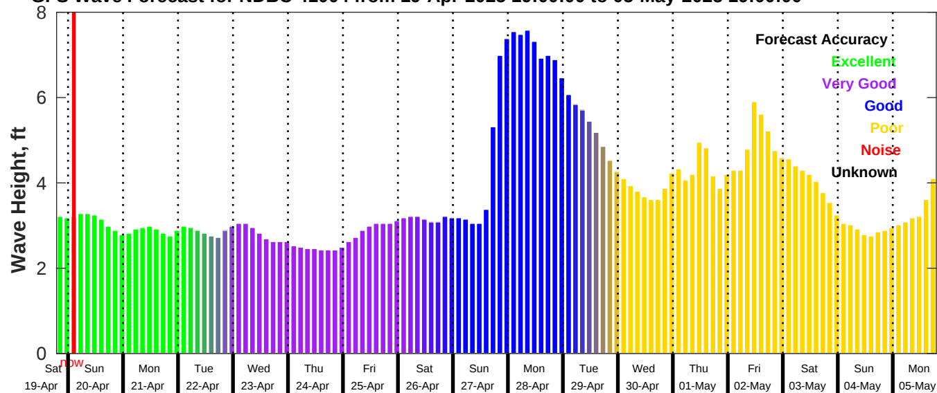
GFS Wave Forecast for NDBC 41004 from 19-Apr-2025 19:00:00 to 05-May-2025 19:00:00
