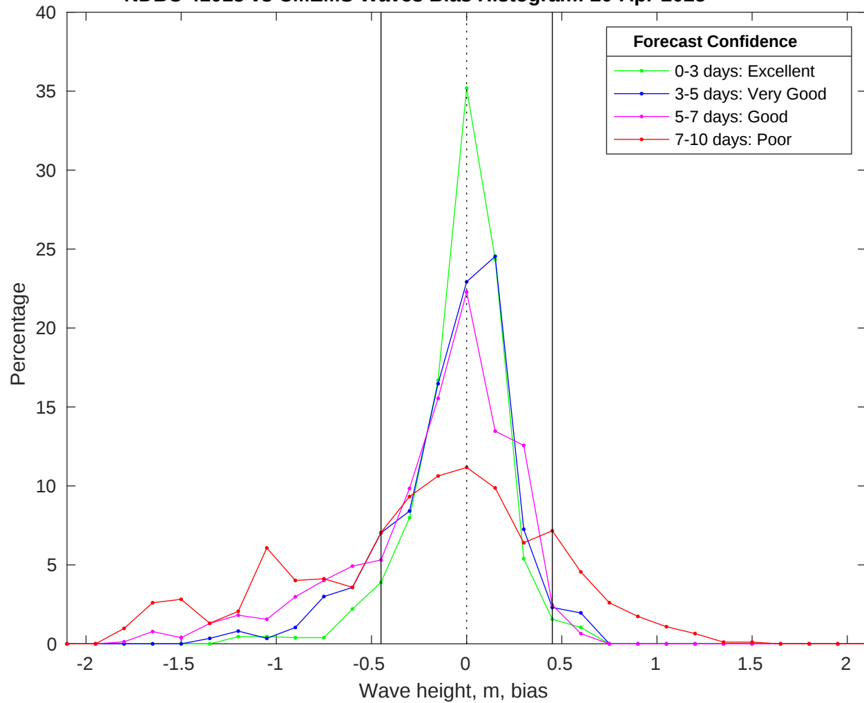
NDBC 41013 vs CMEMS Waves Bias Histogram: 20-Apr-2025
