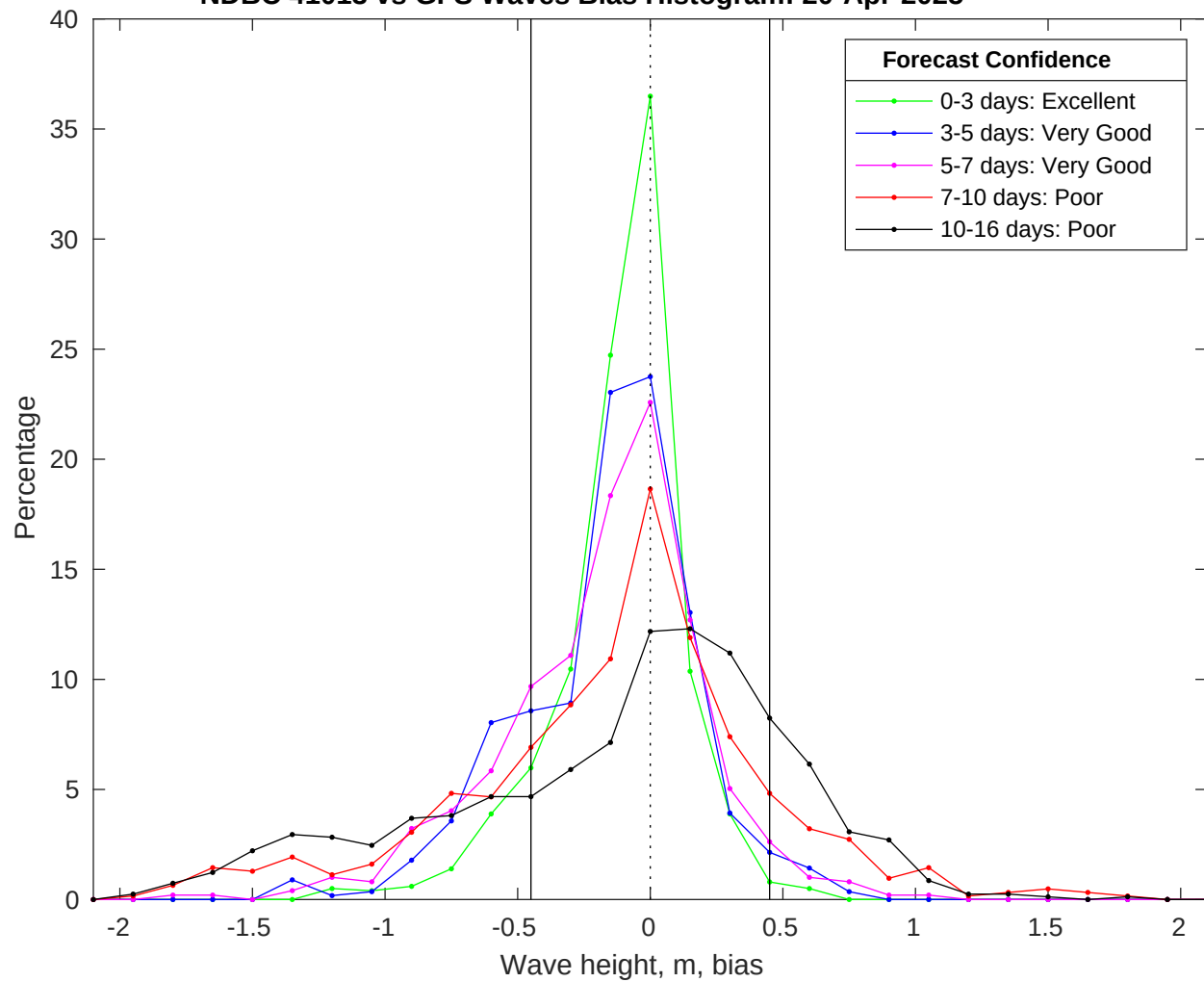
NDBC 41013 vs GFS Waves Bias Histogram: 20-Apr-2025
