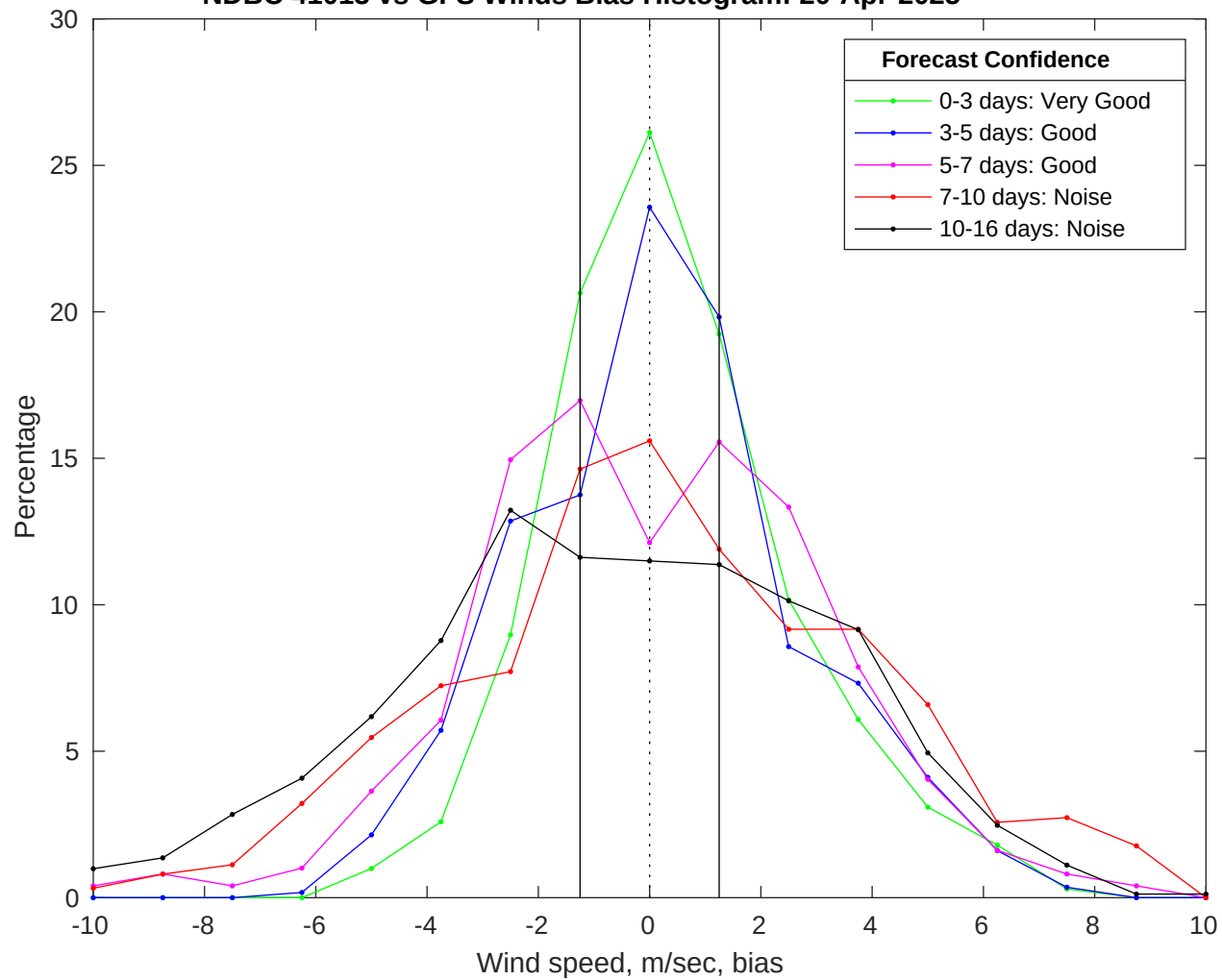
NDBC 41013 vs GFS Winds Bias Histogram: 20-Apr-2025
