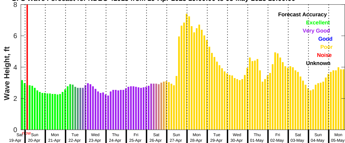
GFS Wave Forecast for NDBC 41013 from 19-Apr-2025 19:00:00 to 05-May-2025 19:00:00
