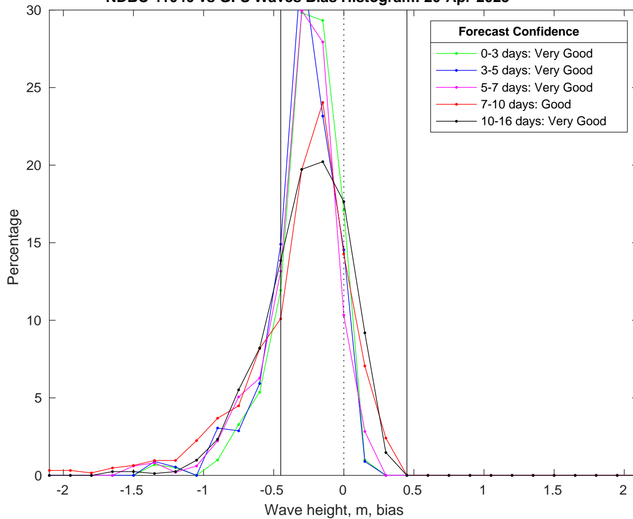
NDBC 41040 vs GFS Waves Bias Histogram: 20-Apr-2025
