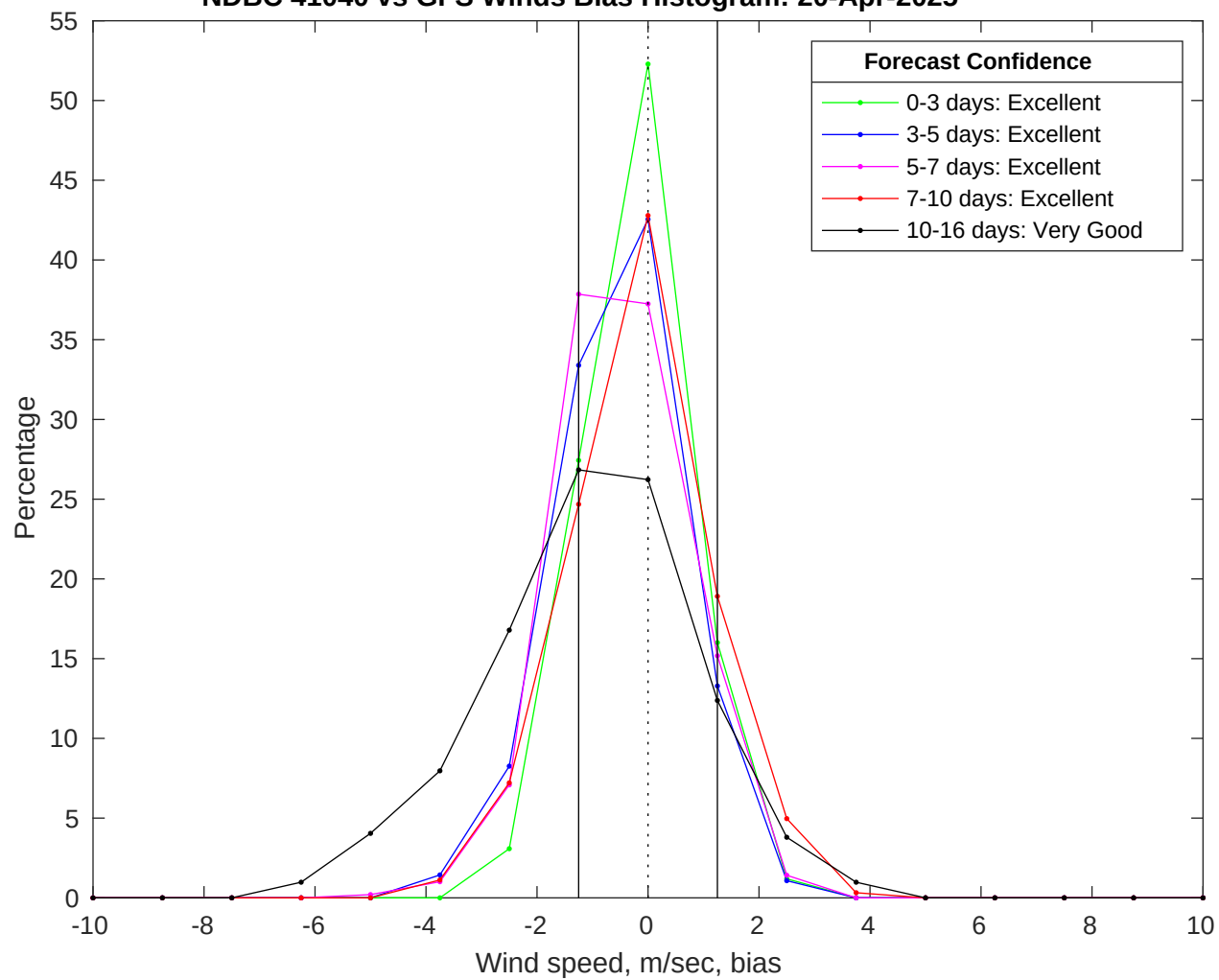
NDBC 41040 vs GFS Winds Bias Histogram: 20-Apr-2025
