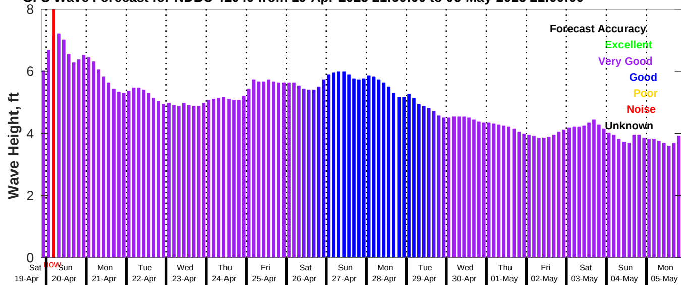
GFS Wave Forecast for NDBC 41040 from 19-Apr-2025 21:00:00 to 05-May-2025 21:00:00
