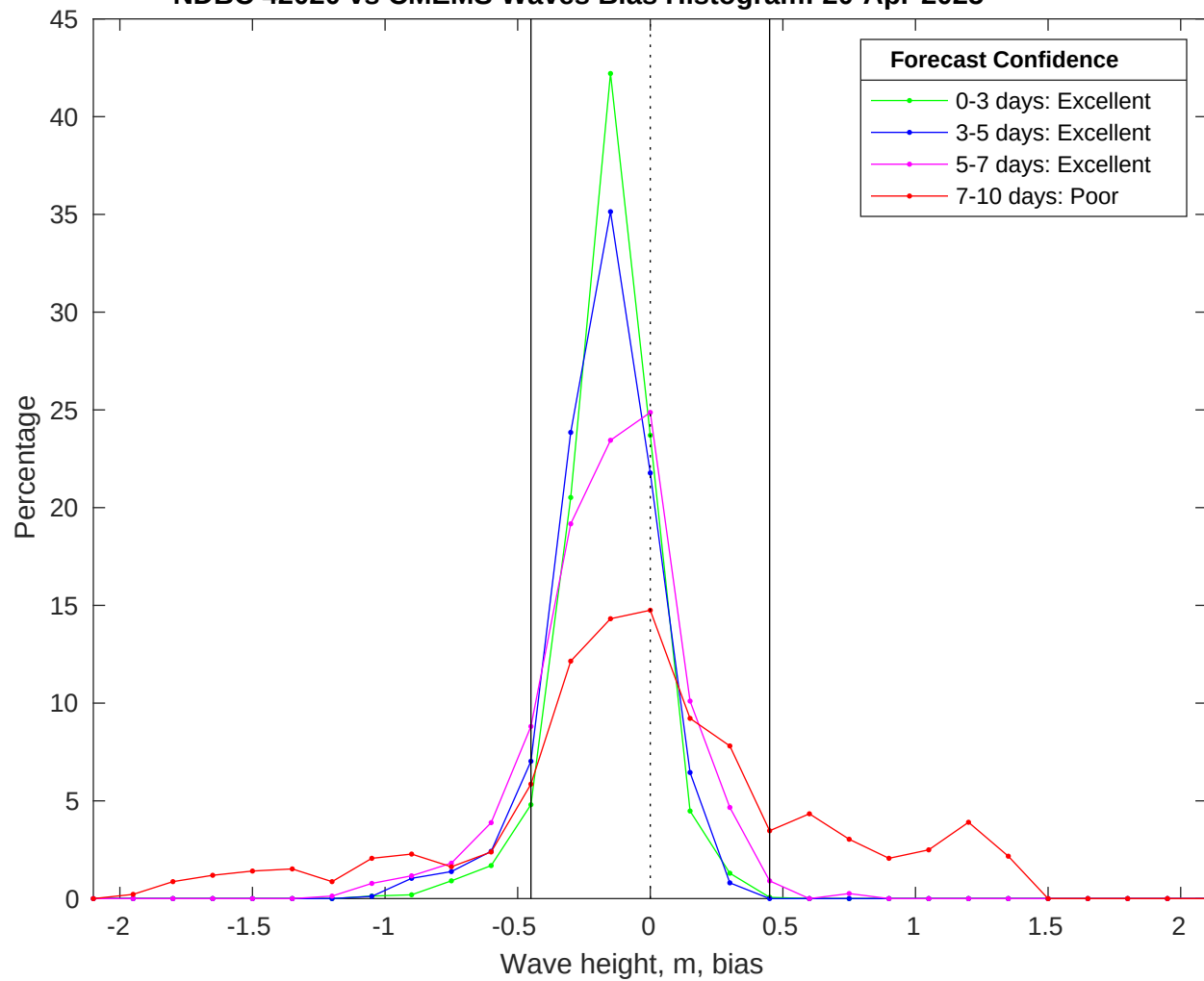
NDBC 42020 vs CMEMS Waves Bias Histogram: 20-Apr-2025
