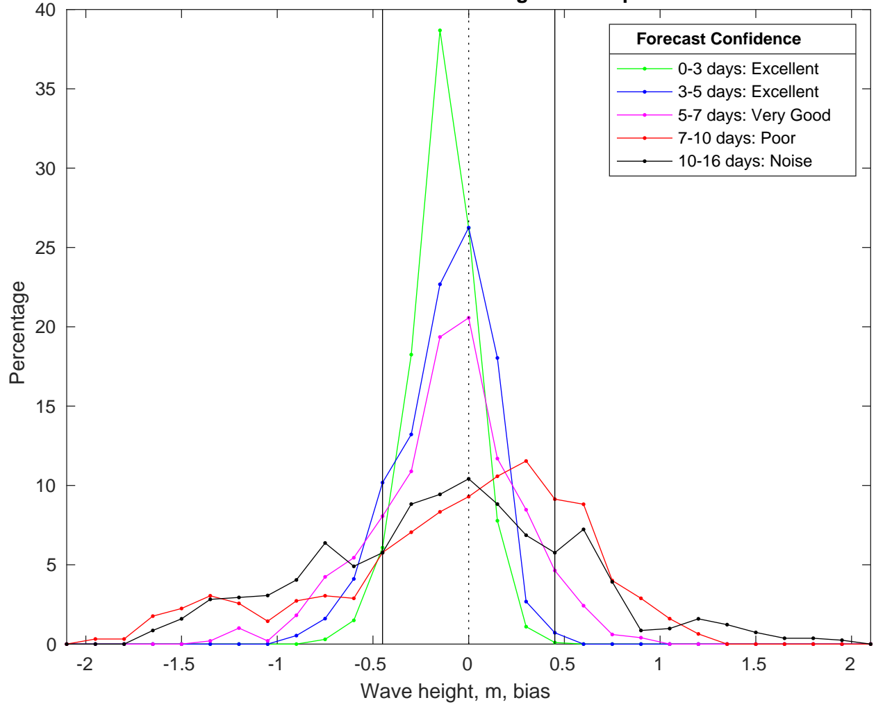
NDBC 42020 vs GFS Waves Bias Histogram: 20-Apr-2025
