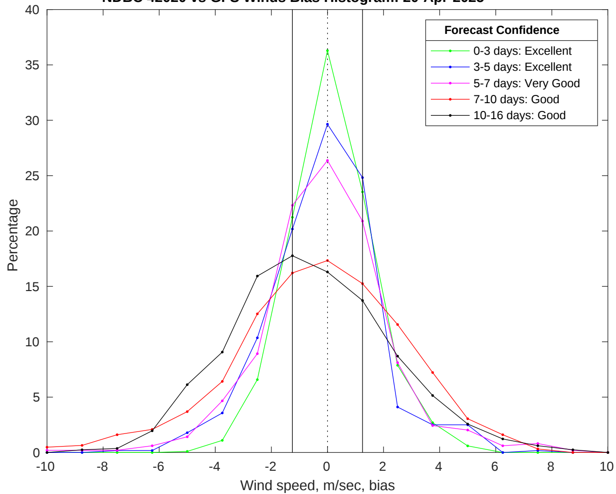
NDBC 42020 vs GFS Winds Bias Histogram: 20-Apr-2025
