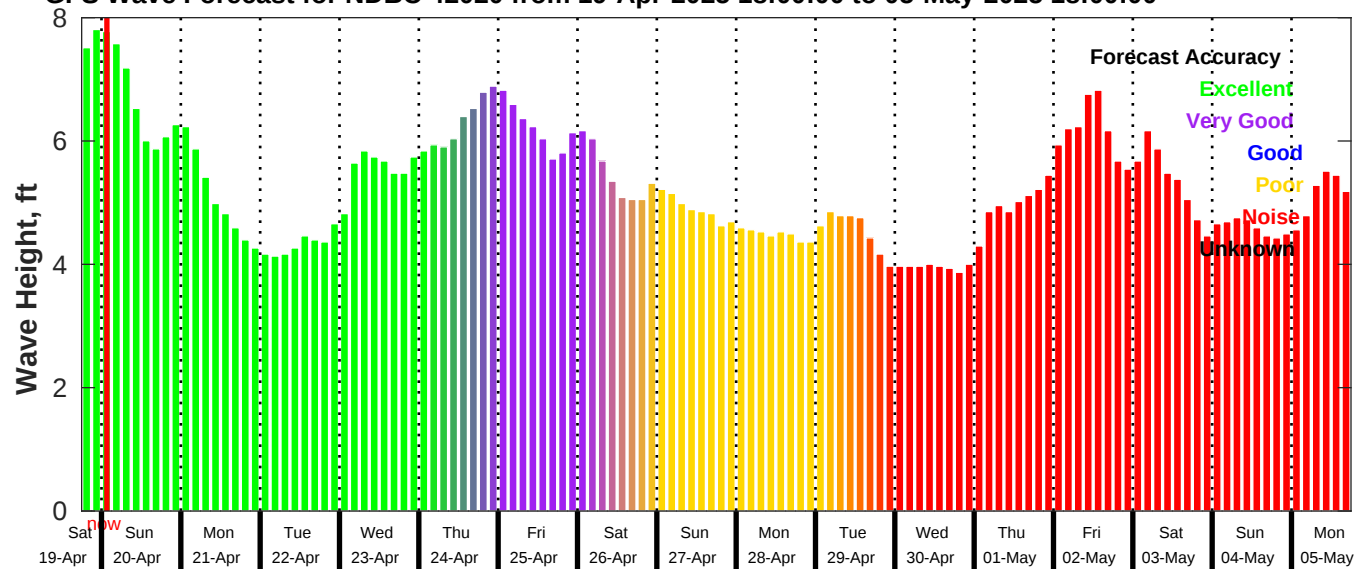
GFS Wave Forecast for NDBC 42020 from 19-Apr-2025 18:00:00 to 05-May-2025 18:00:00
