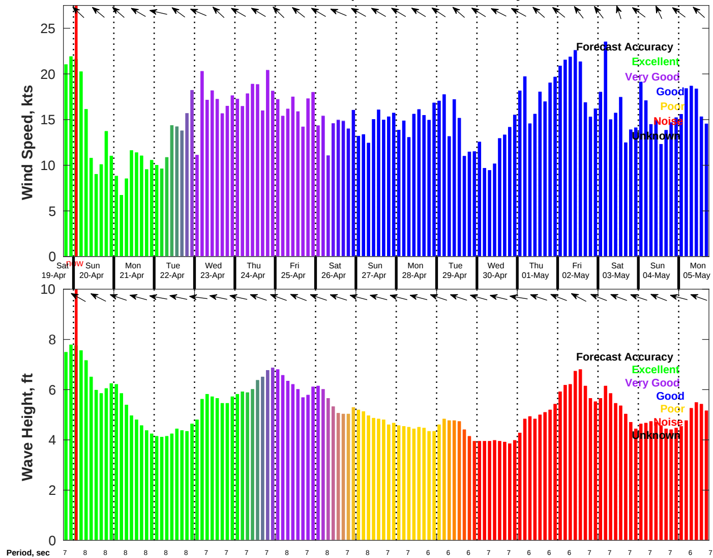
Wind & Wave Forecast for NDBC 42020 from 19-Apr-2025 18:00:00 to 05-May-2025 18:00:00
