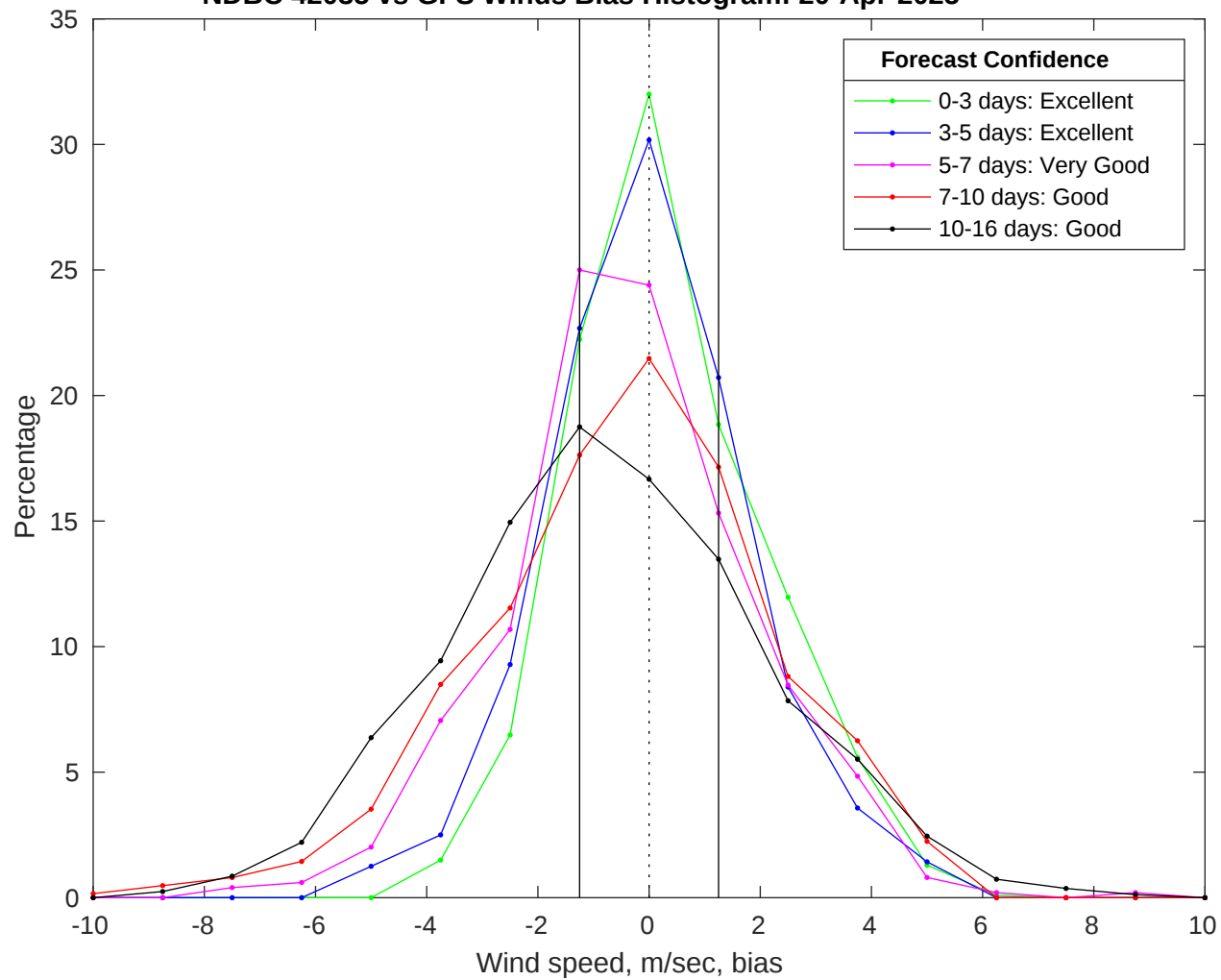
NDBC 42035 vs GFS Winds Bias Histogram: 20-Apr-2025
