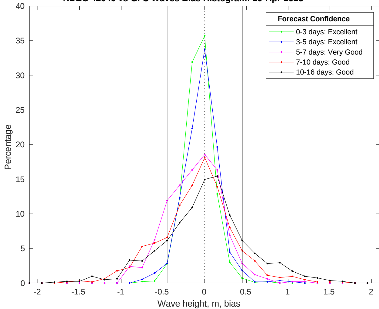
NDBC 42040 vs GFS Waves Bias Histogram: 20-Apr-2025
