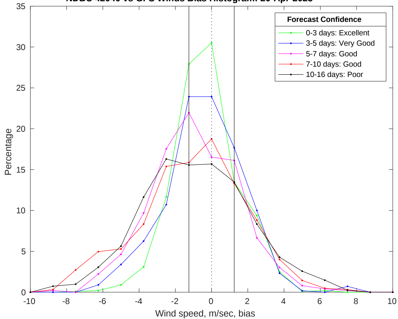
NDBC 42040 vs GFS Winds Bias Histogram: 20-Apr-2025
