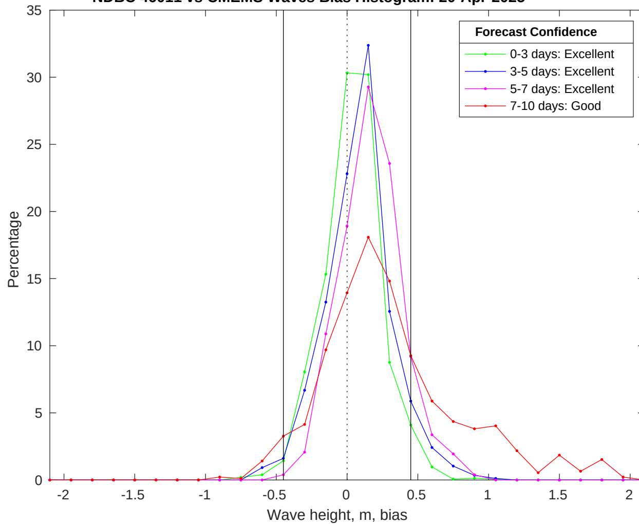
NDBC 46011 vs CMEMS Waves Bias Histogram: 20-Apr-2025
