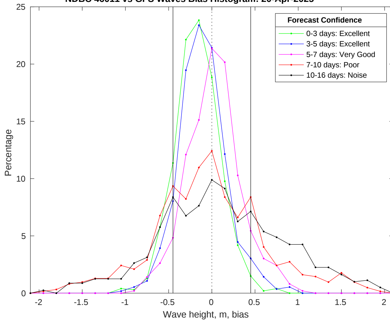
NDBC 46011 vs GFS Waves Bias Histogram: 20-Apr-2025
