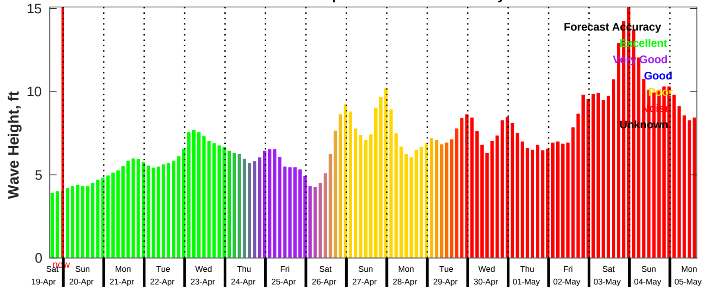
GFS Wave Forecast for NDBC 46011 from 19-Apr-2025 16:00:00 to 05-May-2025 16:00:00
