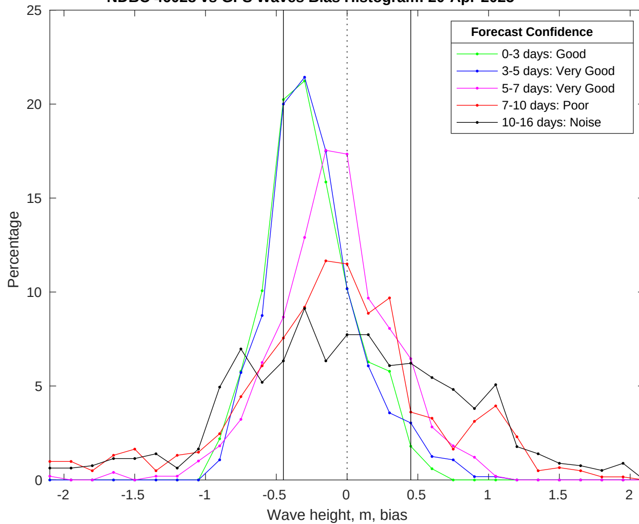
NDBC 46028 vs GFS Waves Bias Histogram: 20-Apr-2025
