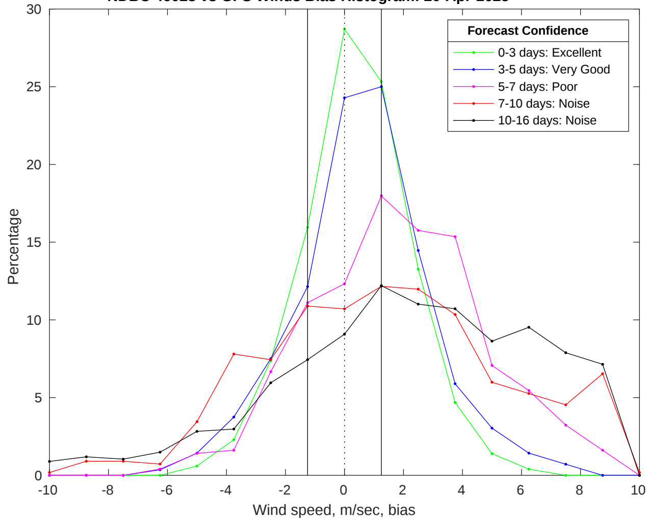
NDBC 46028 vs GFS Winds Bias Histogram: 20-Apr-2025
