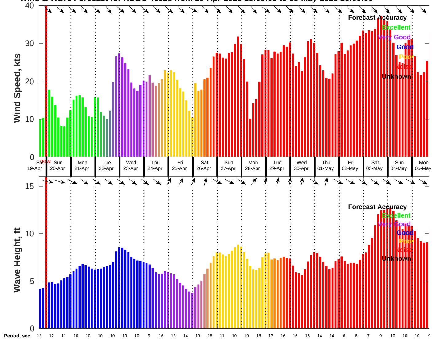
Wind & Wave Forecast for NDBC 46028 from 19-Apr-2025 16:00:00 to 05-May-2025 16:00:00
