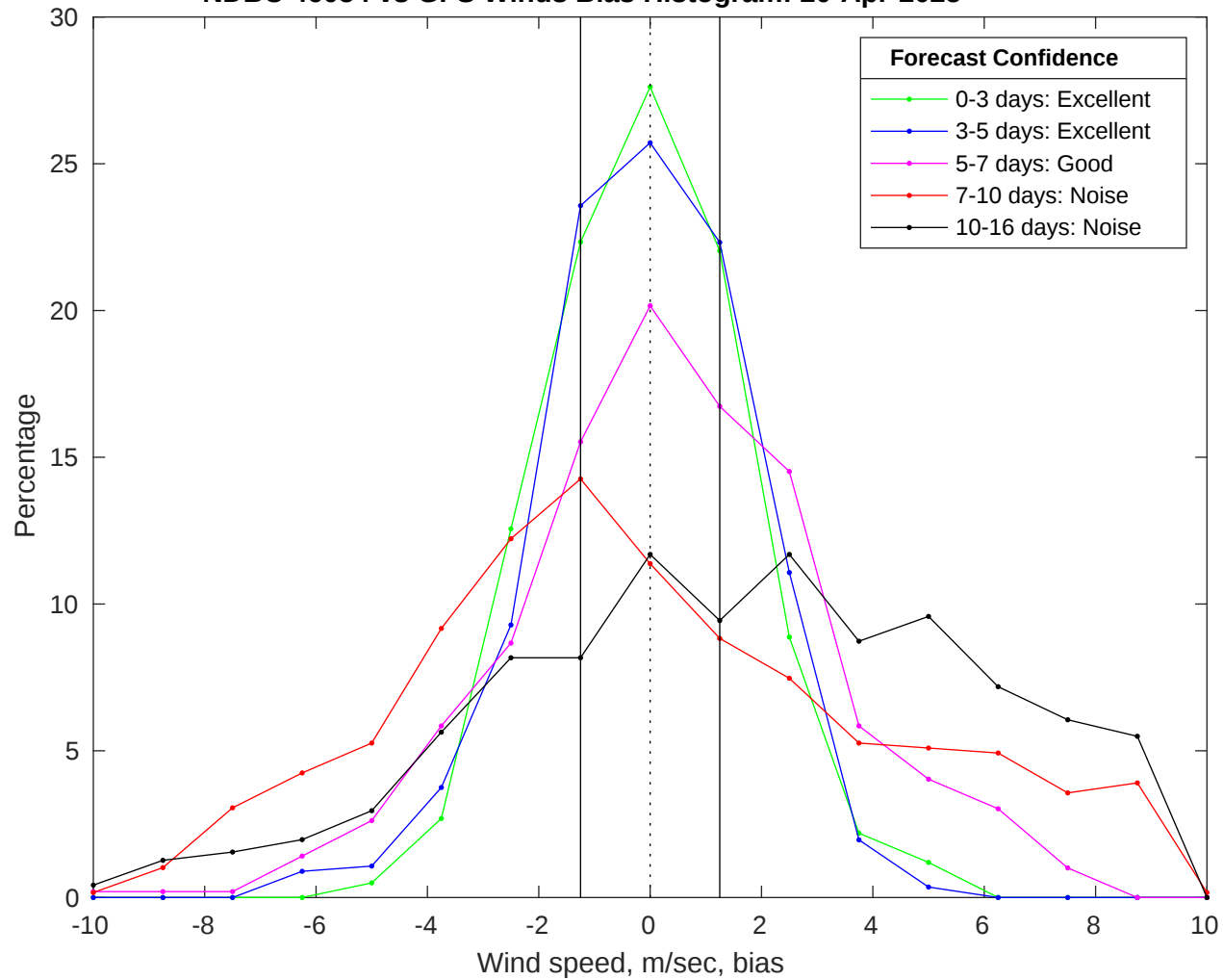
NDBC 46054 vs GFS Winds Bias Histogram: 20-Apr-2025
