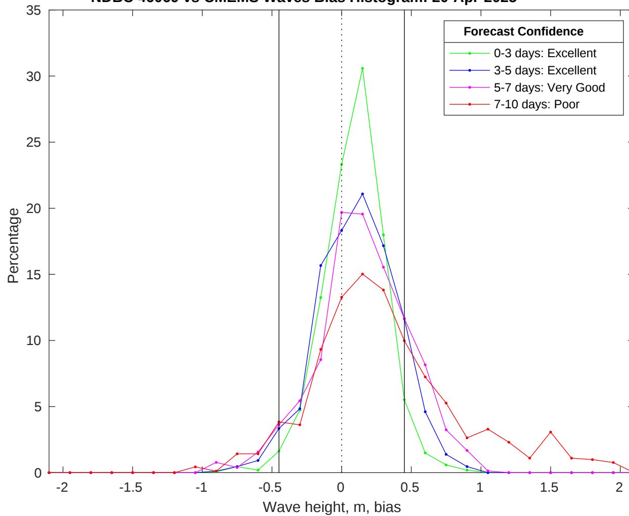
NDBC 46069 vs CMEMS Waves Bias Histogram: 20-Apr-2025
