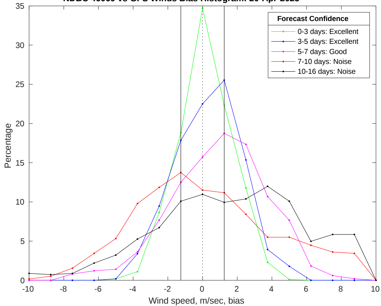
NDBC 46069 vs GFS Winds Bias Histogram: 20-Apr-2025
