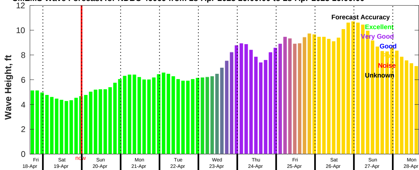
CMEMS Wave Forecast for NDBC 46069 from 18-Apr-2025 16:00:00 to 28-Apr-2025 16:00:00
