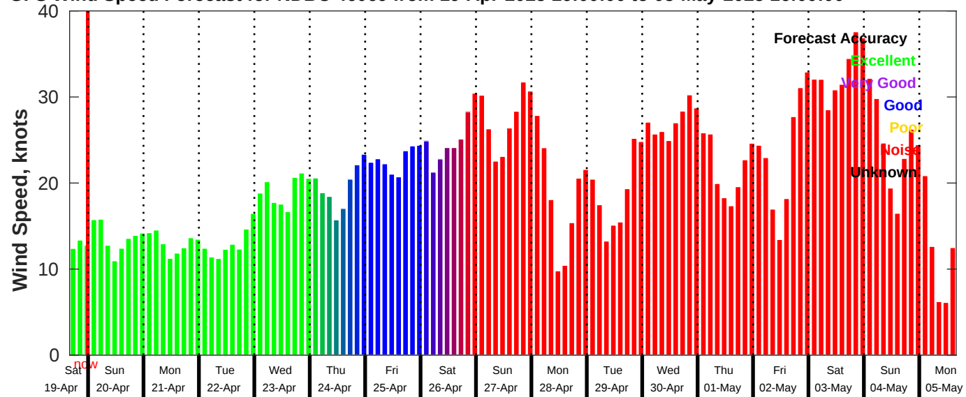
GFS Wind Speed Forecast for NDBC 46069 from 19-Apr-2025 16:00:00 to 05-May-2025 16:00:00
