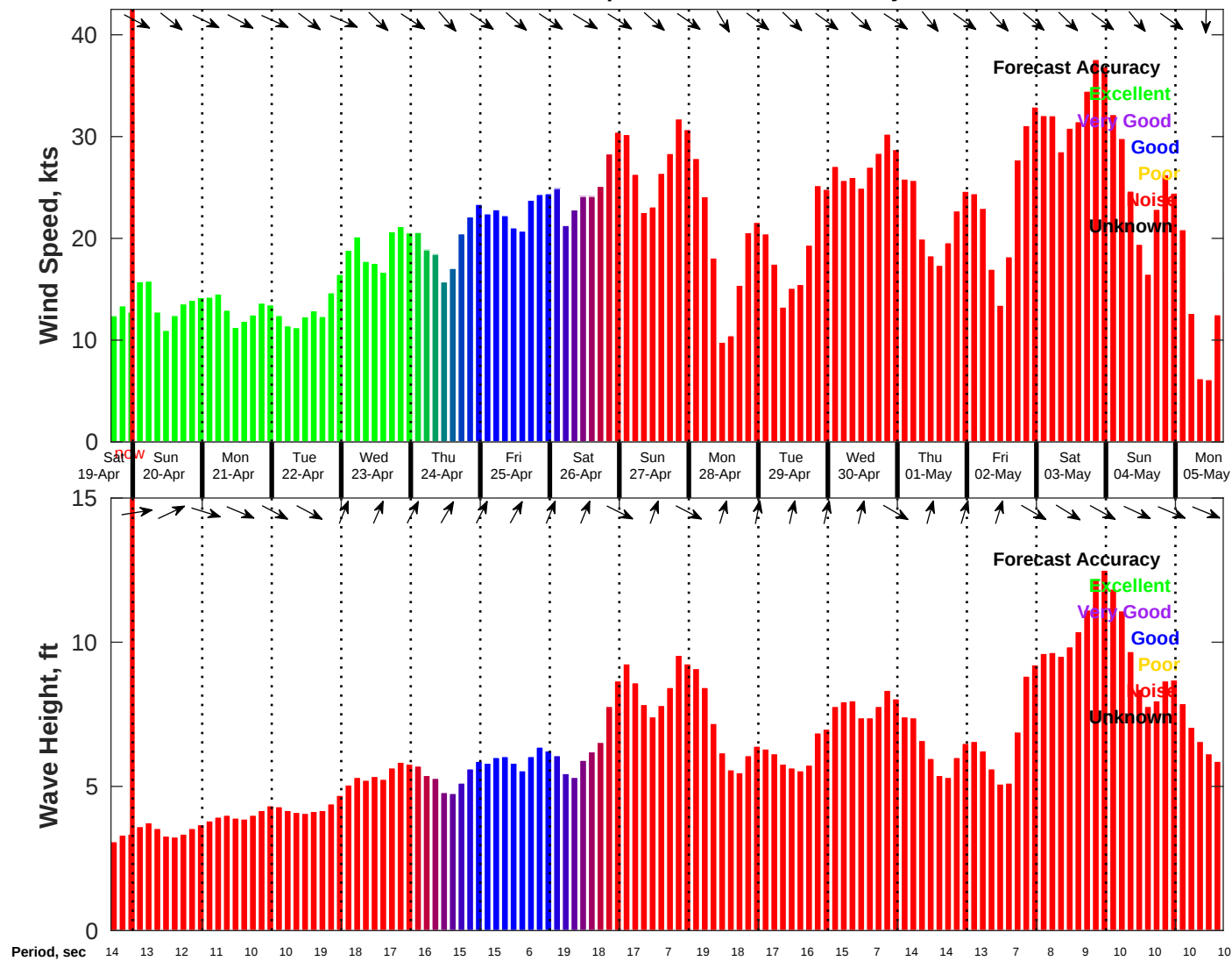
Wind & Wave Forecast for NDBC 46069 from 19-Apr-2025 16:00:00 to 05-May-2025 16:00:00
