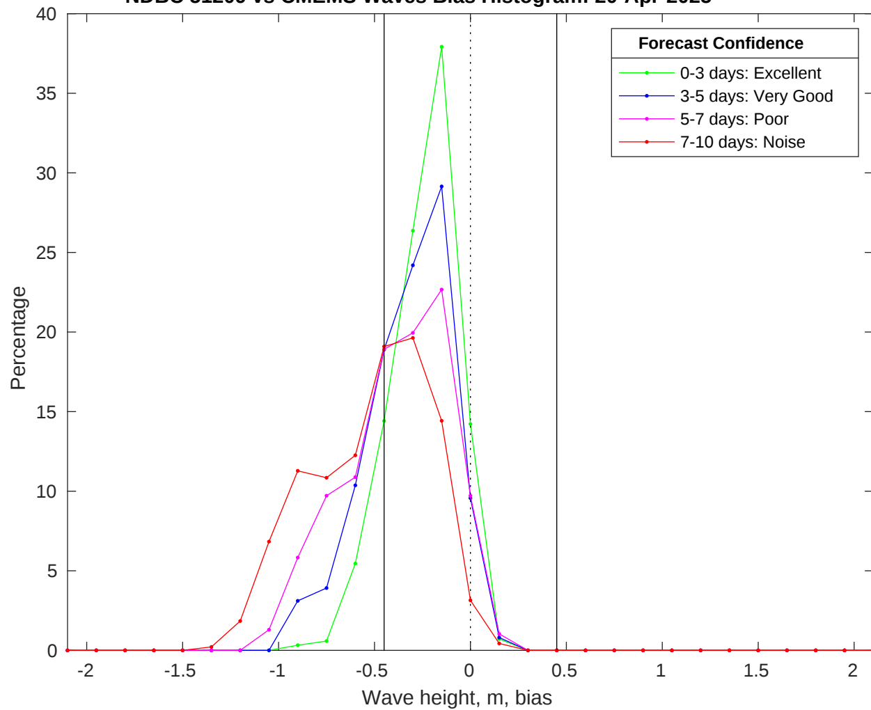
NDBC 51209 vs CMEMS Waves Bias Histogram: 20-Apr-2025
