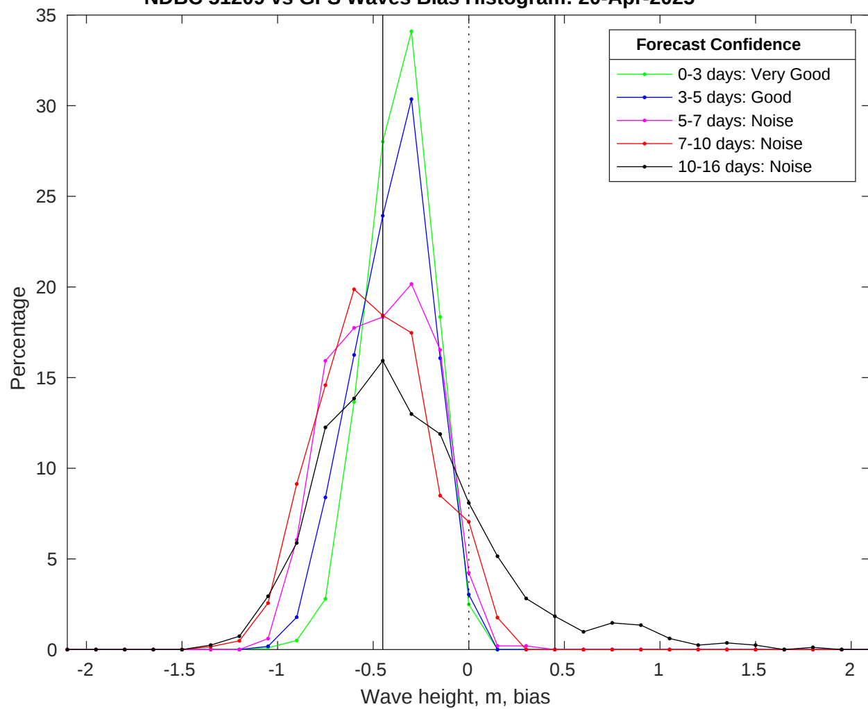
NDBC 51209 vs GFS Waves Bias Histogram: 20-Apr-2025
