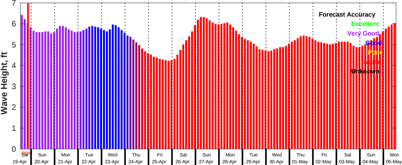
GFS Wave Forecast for NDBC 51209 from 19-Apr-2025 13:00:00 to 05-May-2025 13:00:00
