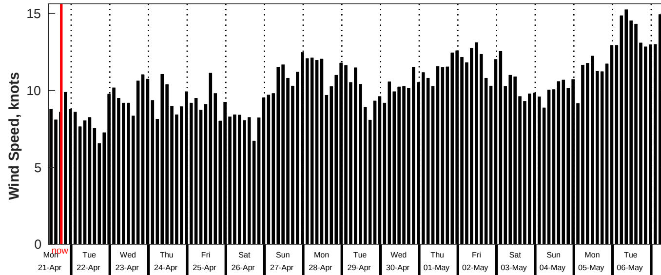
GFS Wind Speed Forecast for NDBC 52211 from 20-Apr-2025 10:00:00 to 06-May-2025 10:00:00
