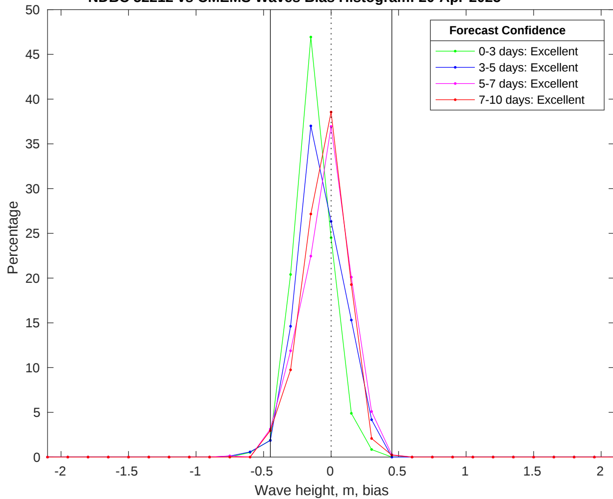
NDBC 52212 vs CMEMS Waves Bias Histogram: 20-Apr-2025
