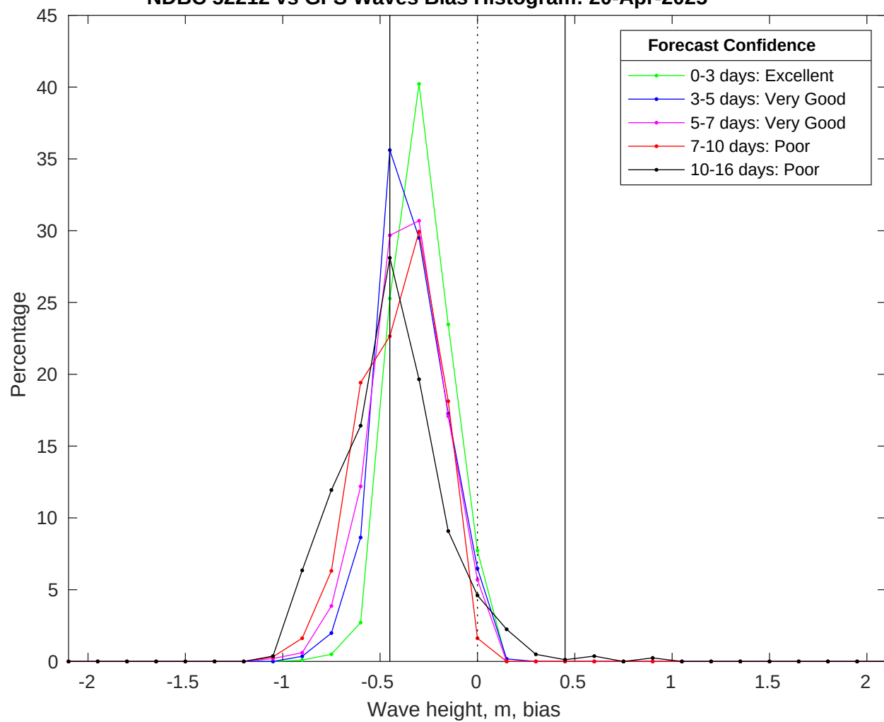
NDBC 52212 vs GFS Waves Bias Histogram: 20-Apr-2025
