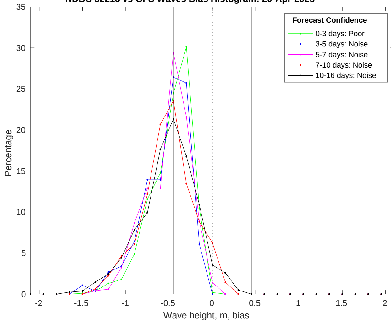
NDBC 52213 vs GFS Waves Bias Histogram: 20-Apr-2025
