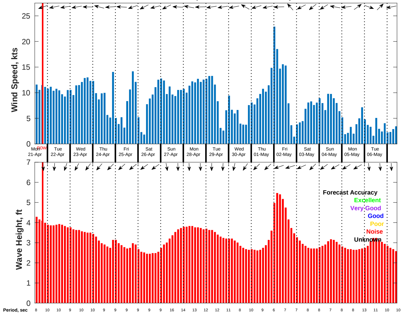
Wind & Wave Forecast for NDBC 52213 from 20-Apr-2025 11:00:00 to 06-May-2025 11:00:00
