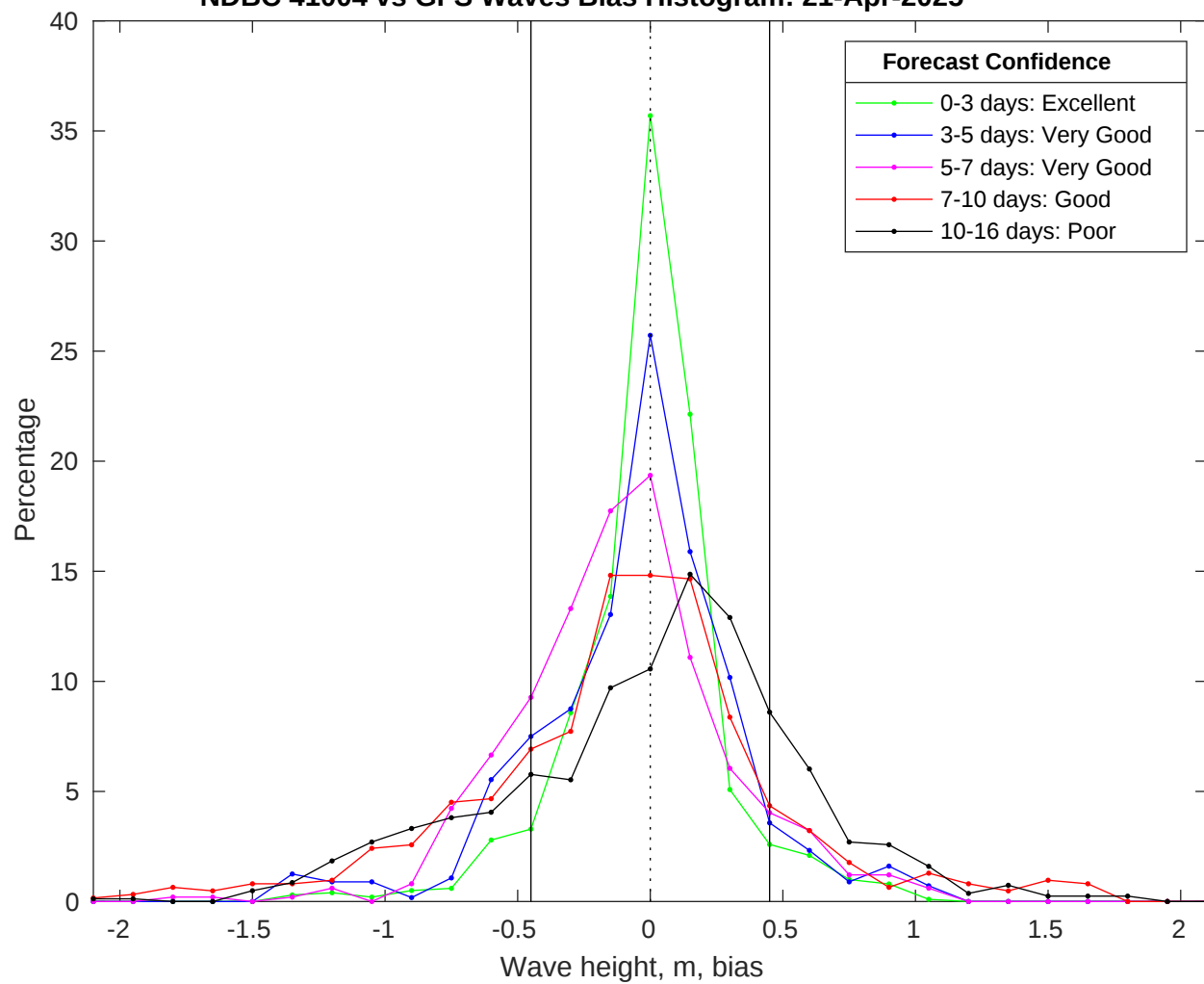
NDBC 41004 vs GFS Waves Bias Histogram: 21-Apr-2025
