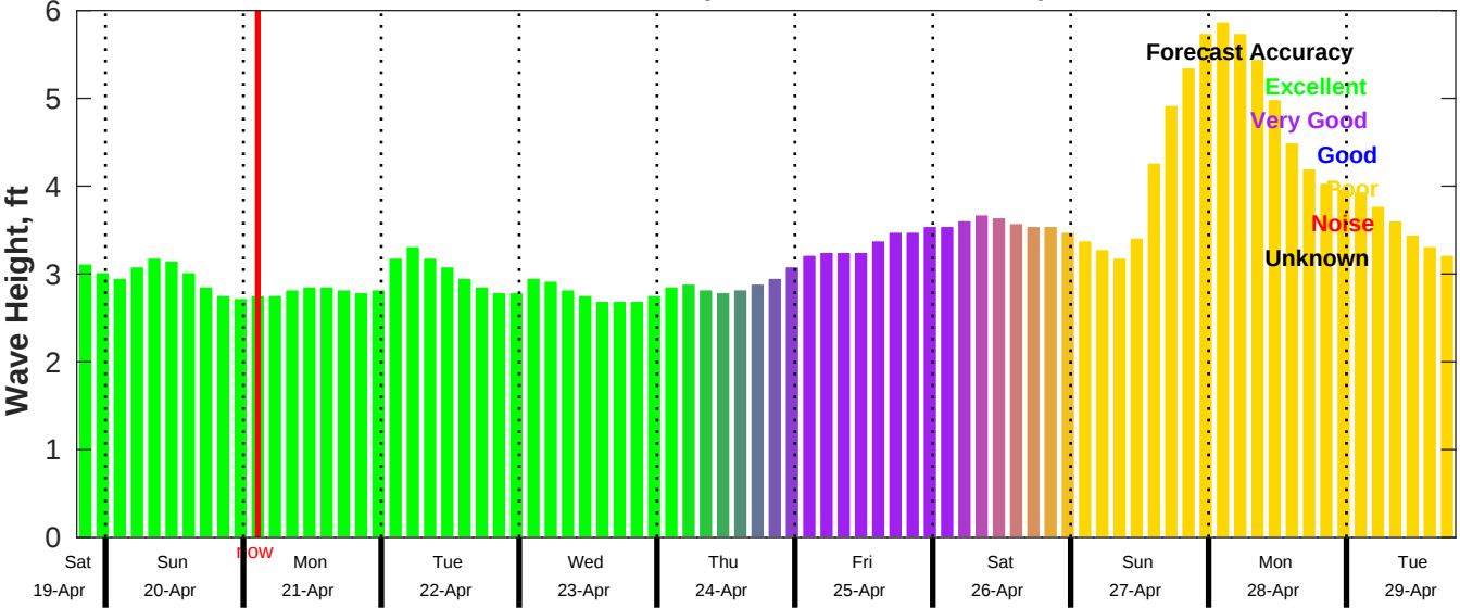
CMEMS Wave Forecast for NDBC 41004 from 19-Apr-2025 19:00:00 to 29-Apr-2025 19:00:00
