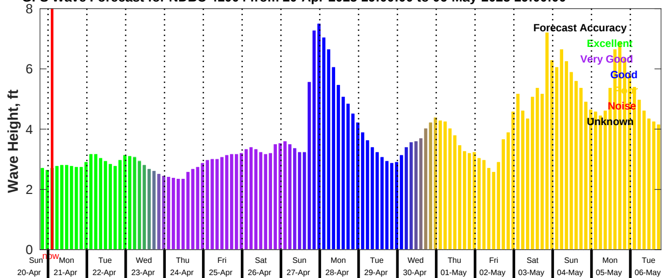
GFS Wave Forecast for NDBC 41004 from 20-Apr-2025 19:00:00 to 06-May-2025 19:00:00
