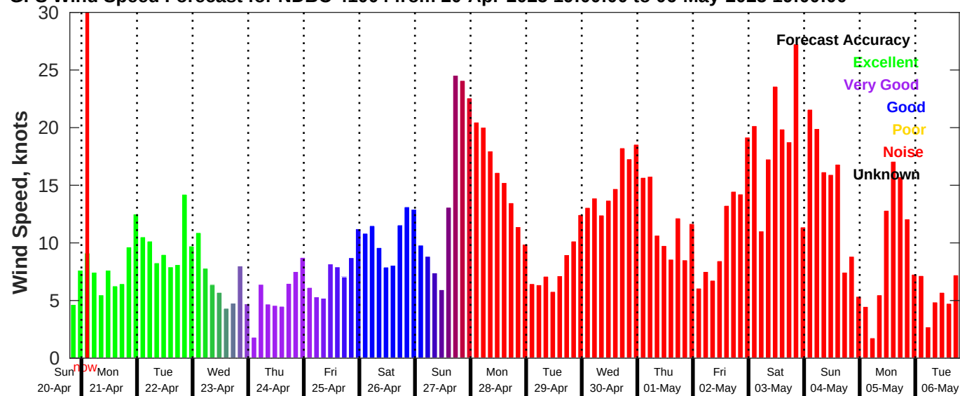
GFS Wind Speed Forecast for NDBC 41004 from 20-Apr-2025 19:00:00 to 06-May-2025 19:00:00
