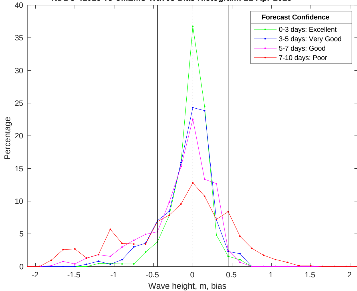
NDBC 41013 vs CMEMS Waves Bias Histogram: 21-Apr-2025
