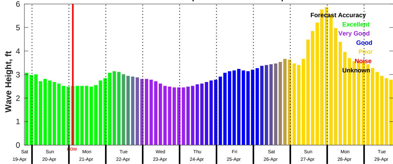
CMEMS Wave Forecast for NDBC 41013 from 19-Apr-2025 19:00:00 to 29-Apr-2025 19:00:00
