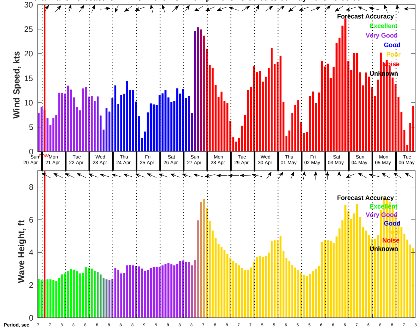
Wind & Wave Forecast for NDBC 41013 from 20-Apr-2025 19:00:00 to 06-May-2025 19:00:00
