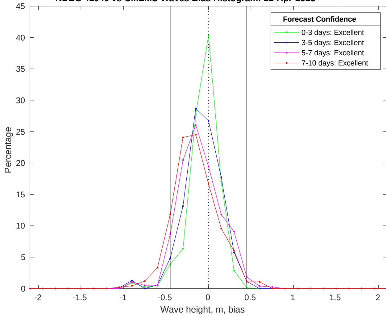
NDBC 41040 vs CMEMS Waves Bias Histogram: 21-Apr-2025
