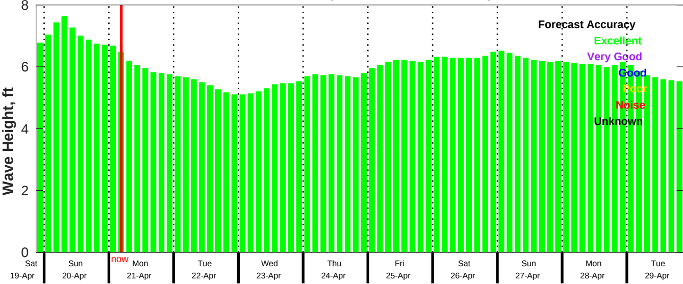
CMEMS Wave Forecast for NDBC 41040 from 19-Apr-2025 21:00:00 to 29-Apr-2025 21:00:00
